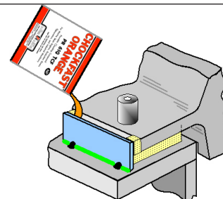
Fig. 8: Pour Chockfast Into Lowest End of Overpour Area
