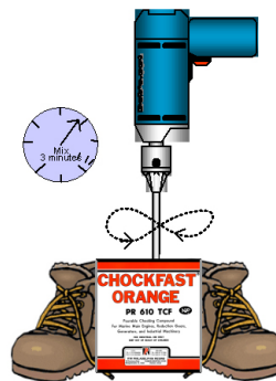
Fig. 7: Mix Resin & Hardener for 3 to 4 minutes
