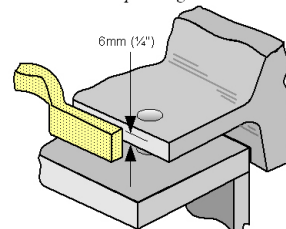
Fig. 1 Trim Foam to Proper Height
