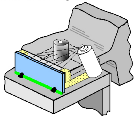
Fig. 5: Seal Front Dam at Bottom & Spray the Inside Face with Release Agent
